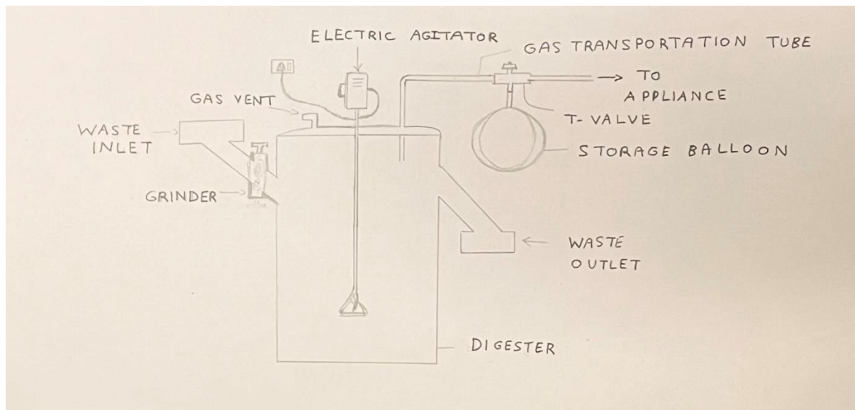
Figure 1: Schematic of Biogas plant
